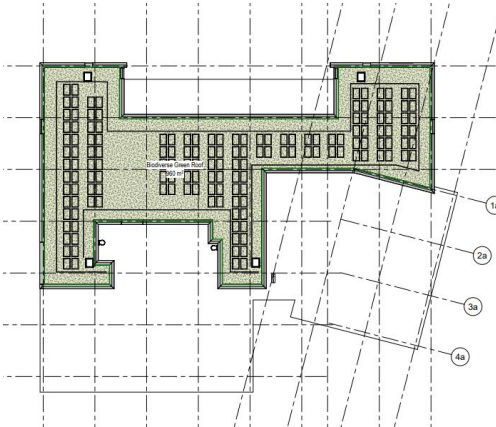
Roof plan:
